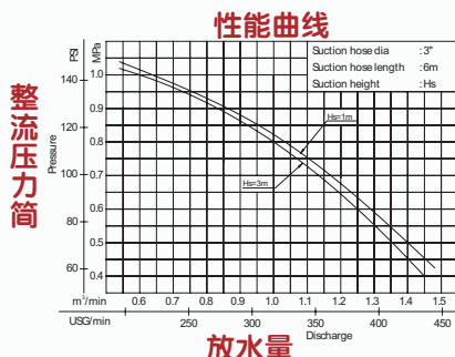
Pumping performance curve
